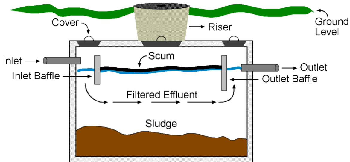
Septic Tank
